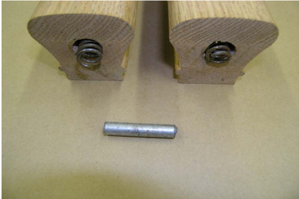
PHOTOGRAPH 1 TEST SPECIMEN COMPONENTS AND CONSTRUCTION
